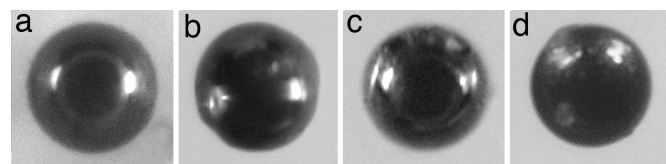
Fig. 2. High-titanomagnetite microspherules from Blackwater Draw, NM ( 120 \mu\text{m} ) (a); Chobot, AB, Canada ( 150 \mu\text{m} ) (b); Gainey, MI ( 90 \mu\text{m} ) (c), and Howard Bay, NC ( 100 \mu\text{m} ) (d).
